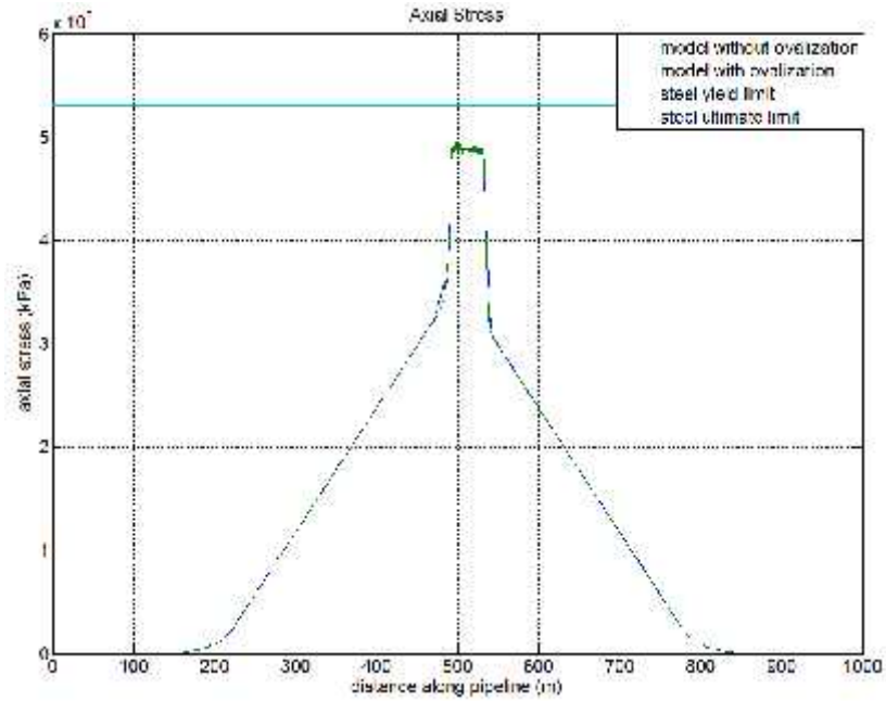
Figure 4 Axial stress
