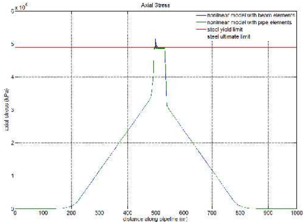
Figure 7 Axial stress and strain around the fault zone
