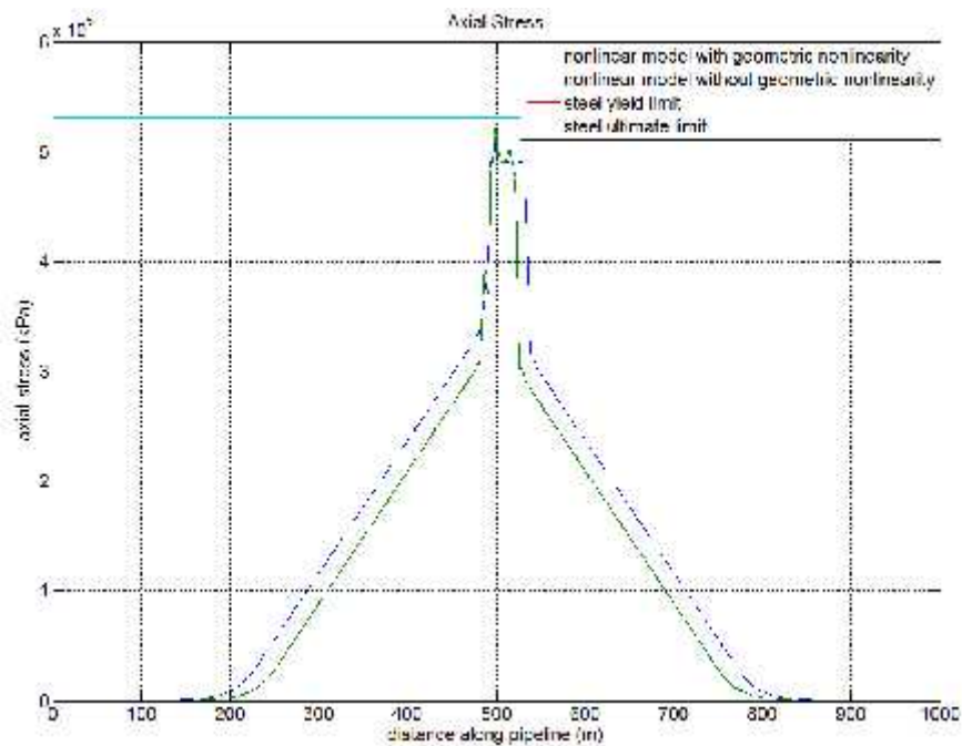
Figure 2 Axial stress
