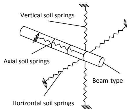
Figure 1 Model used for analyses with the Finite Element Method
